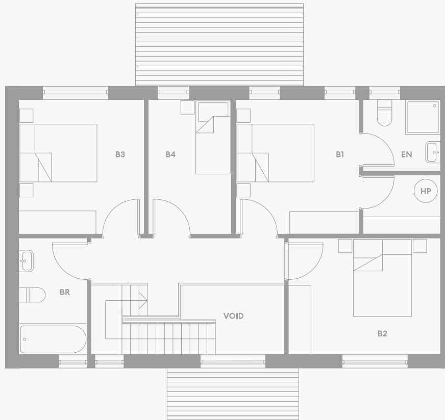
FIRST FLOOR
